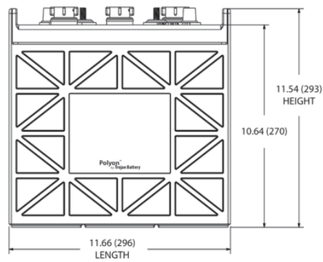
BATTERY DIMENSIONS (shown with DT)
