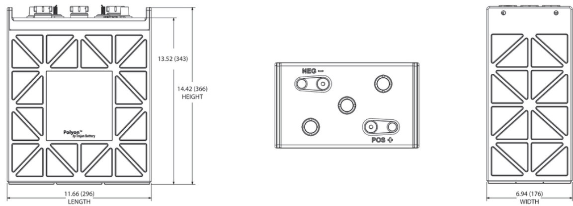
TERMINAL CONFIGURATIONS 6
